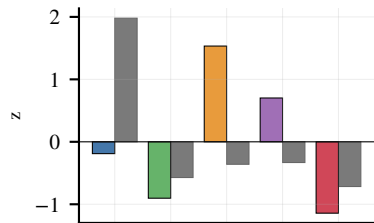
\|W_{OV}\|_F vs BLiMP English r=+0.52
